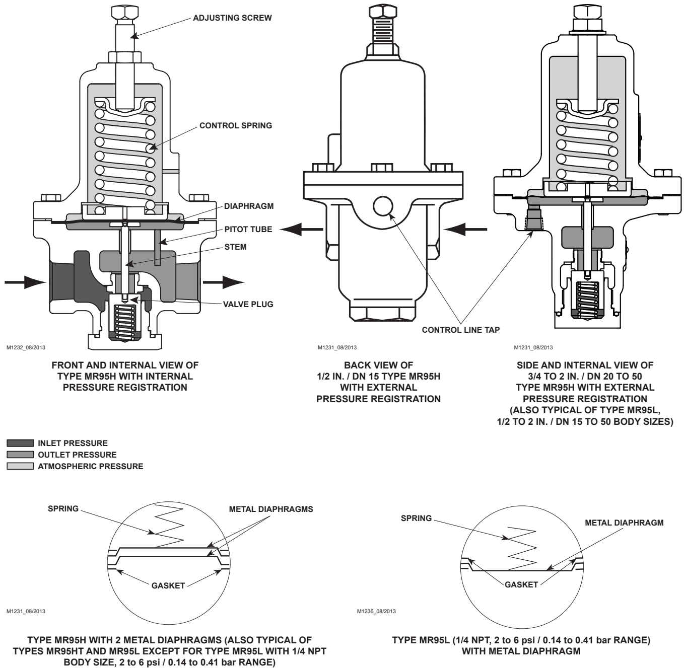
Figure 2. MR95 Series Operational Schematics
