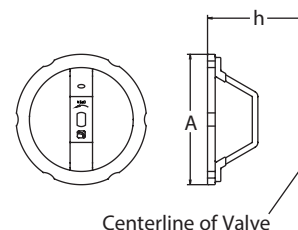
1/2" – 1-1/2" (DN 15 – 40) Series 9000
