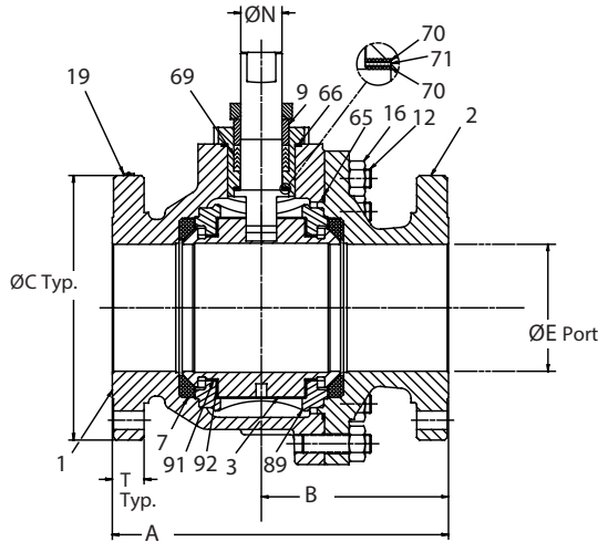
10" & 12" (DN 250 & 300) Class 150 & 300
