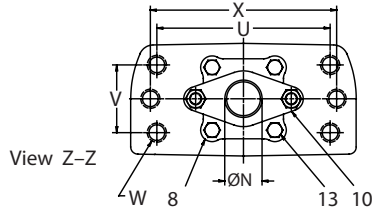
10" & 12" (DN 250 & 300) Class 150 & 300
