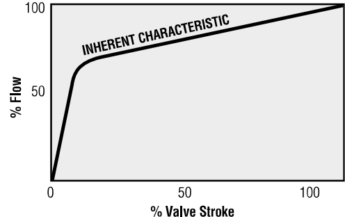
Figure 13: Flow Characteristics
