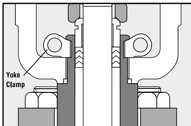
Figure 10: Yoke Clamp
