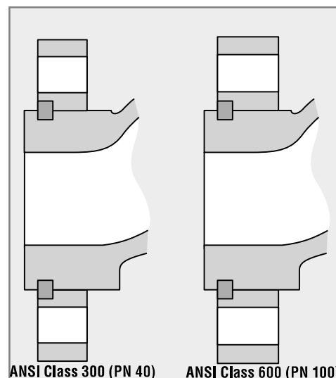
Figure 8: End Flanges
