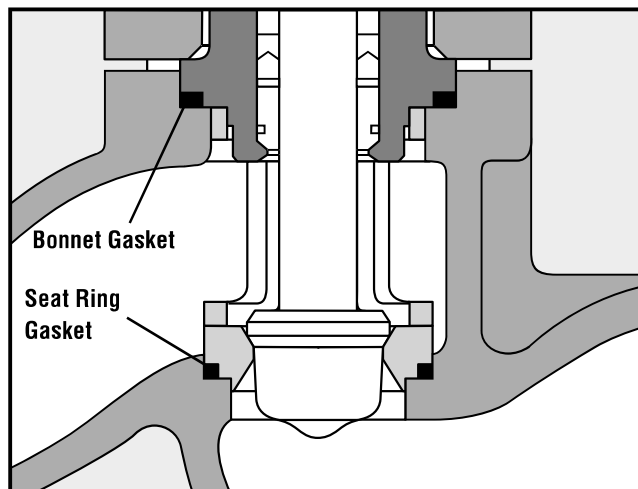
Figure 9: Body Gaskets
