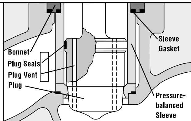
Figure 16: Pressure-balanced Trim
