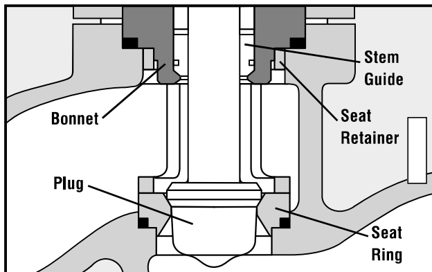
Figure 15: Standard Trim
