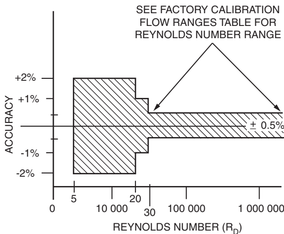
Figure 1. Flowmeter Accuracy for Fluids
