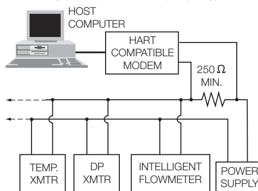
Figure 4. HART Multidrop Topology
