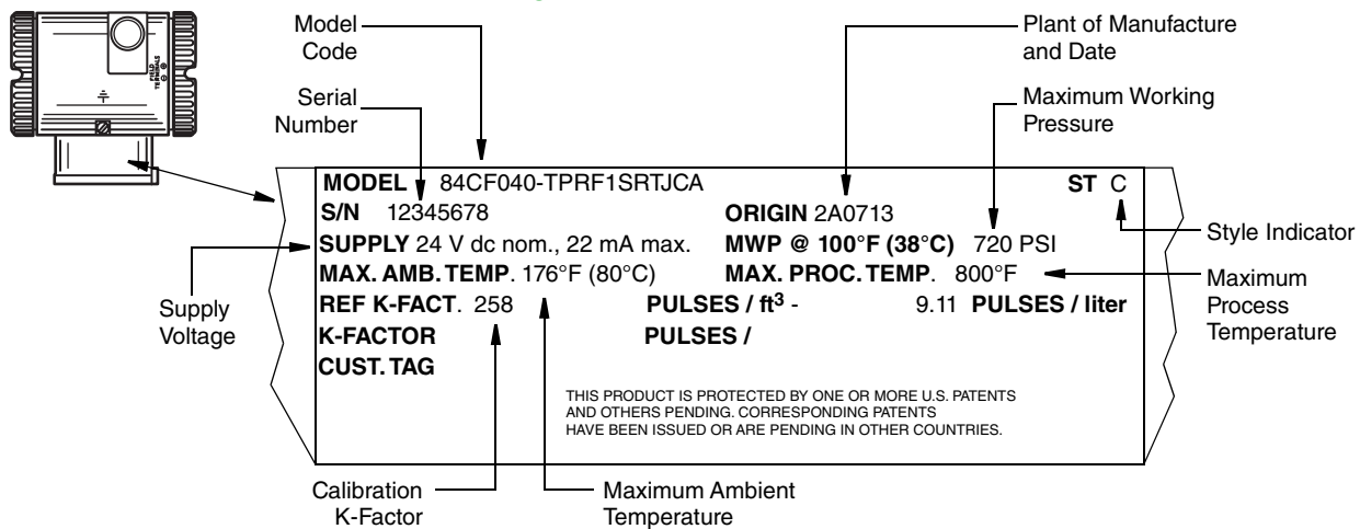
Figure 6. Flowmeter Data Plate
