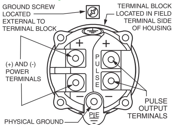
Figure 5. Terminal Block
