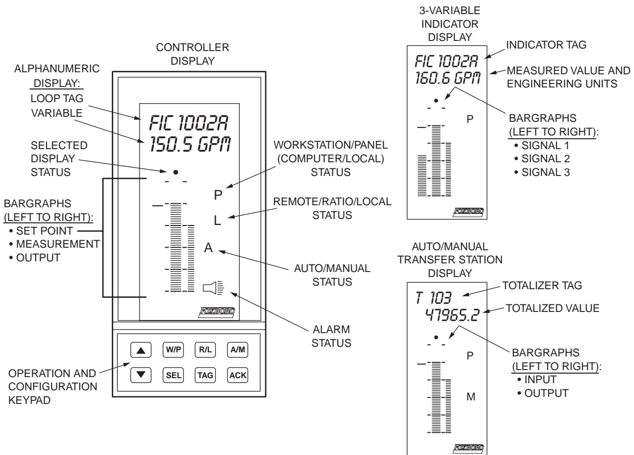
Figure 1. Controller Front Panel
