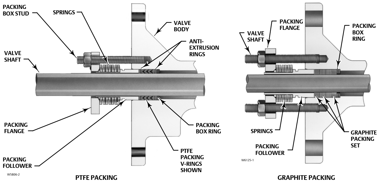
Figure 4. Typical ENVIRO-SEAL Packing Arrangements
