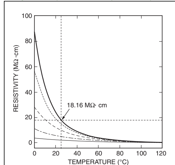
Figure 6. Temperature/Resistivity Relationship
