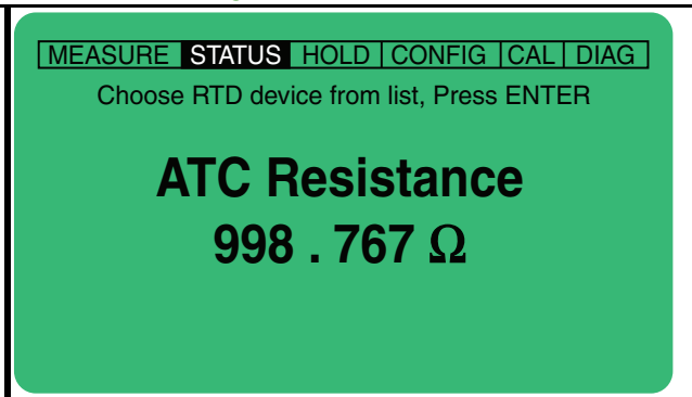
Figure 4. Status Screen
