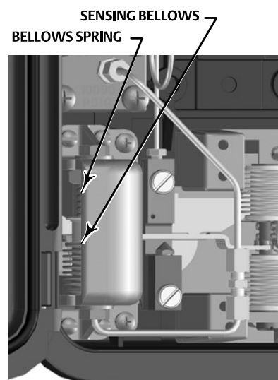
BELLOWS DETAILS
