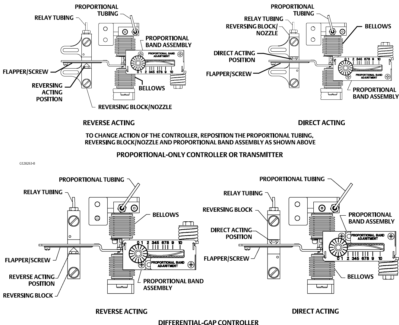
Figure 3. Conversion from Reverse to Direct Action or Proportional to Differential Gap
