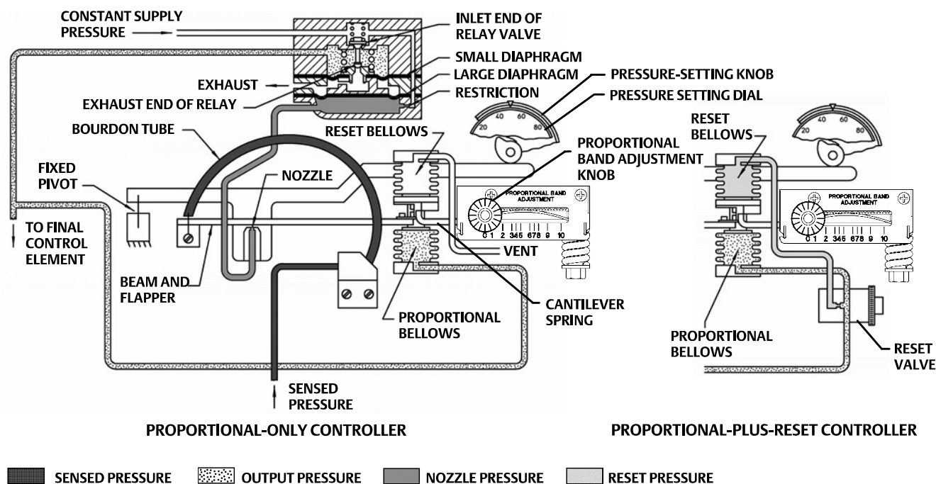
Figure 1. Schematic of Reverse-Acting Proportional-Only and Proportional-Plus-Reset Controllers
